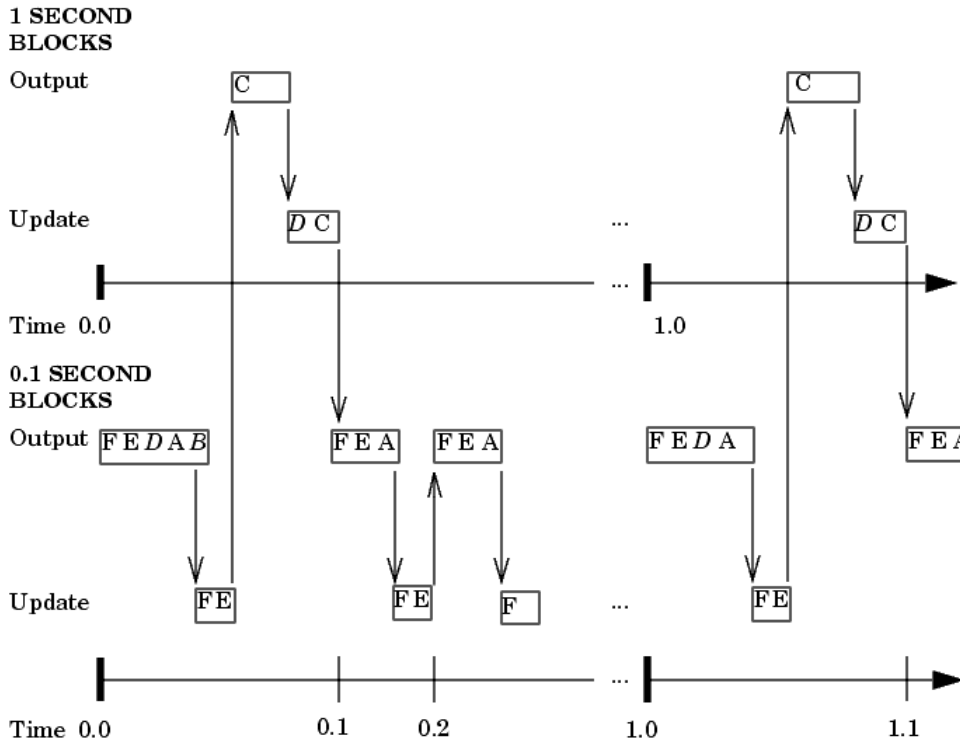
Multitasking Execution of Model in Simulink
