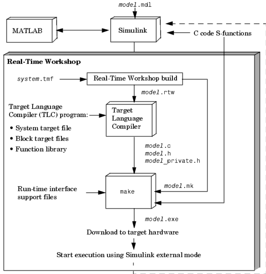
Real-Time Workshop Architecture
