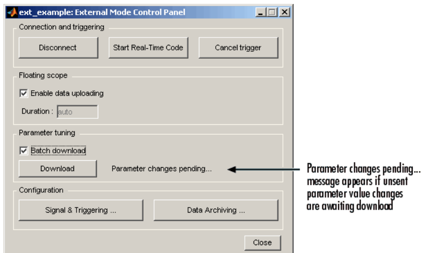
External Mode Control Panel in Batch Download Mode
